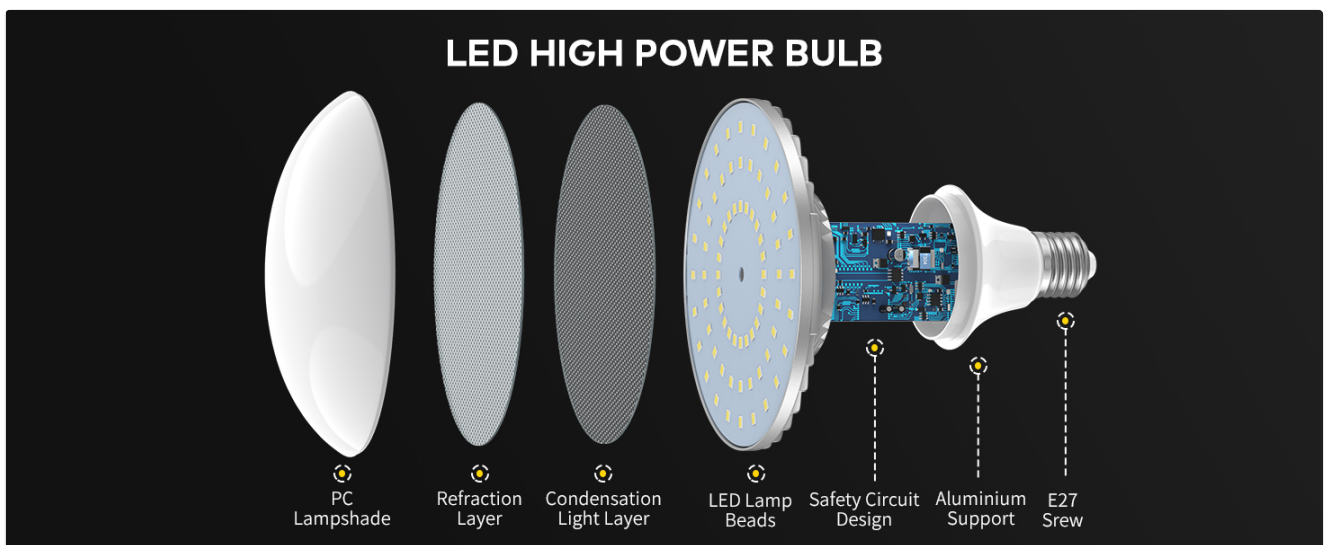
Image: Exploded view diagram of the 50W LED bulb, showing its internal components including the PC lampshade, refraction layer, condensation light layer, LED lamp beads, safety circuit, aluminum support, and E27 screw base.
