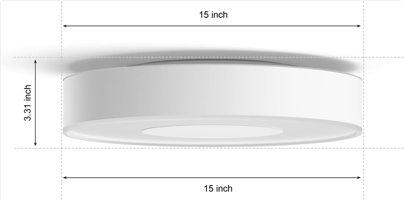
Figure 12: Technical drawing illustrating the dimensions of the Philips Hue Infuse Medium Ceiling Lamp, showing its 15-inch length and width, and 3.31-inch height.
