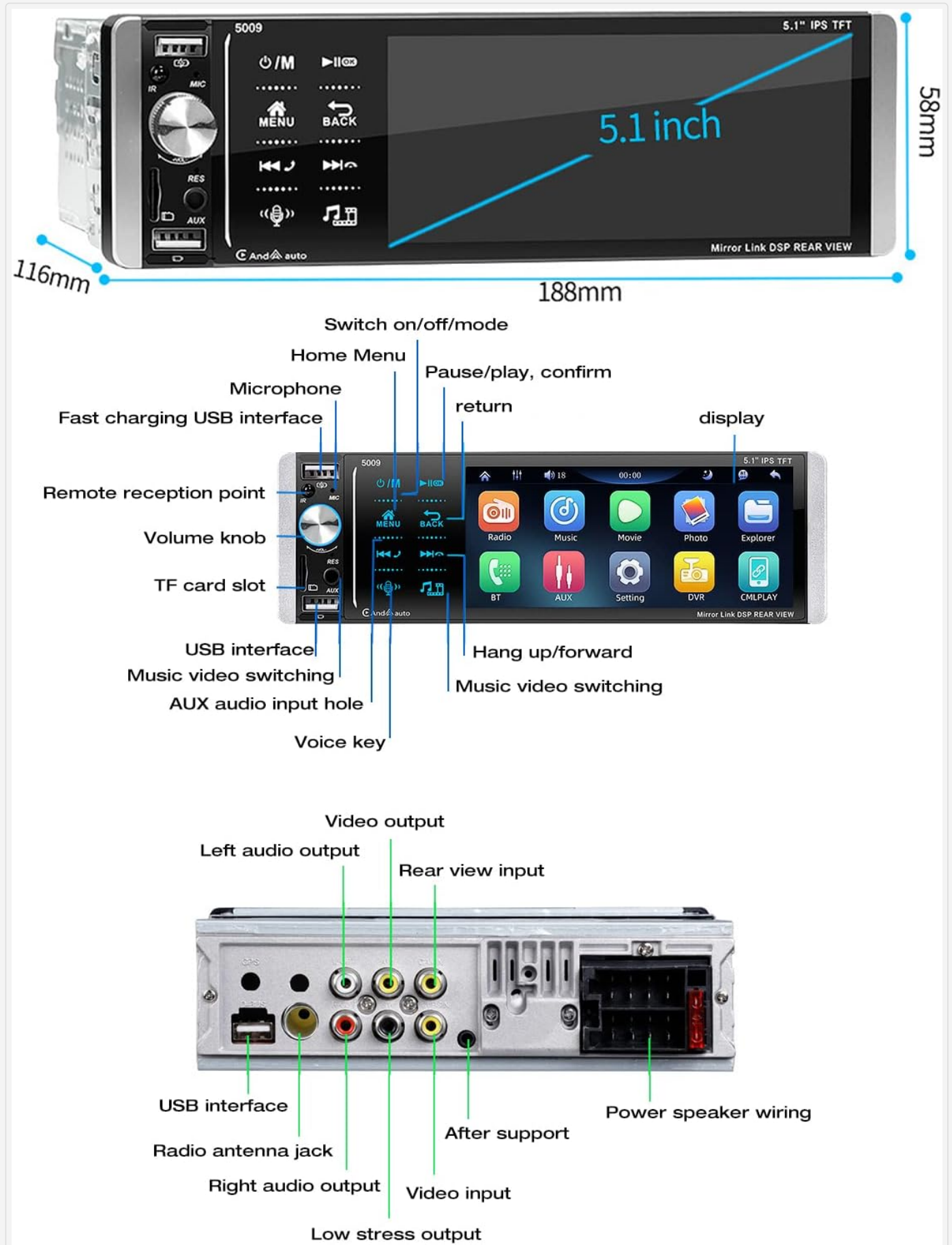
Image 4.1: Detailed diagram illustrating the front panel controls (e.g., volume knob, USB ports, microphone, IR receiver, TF card slot) and rear panel connections (e.g., power speaker wiring, audio outputs, video input, radio antenna jack) of the ASHATA 5.1-inch Single Din MP5 Car Radio.
