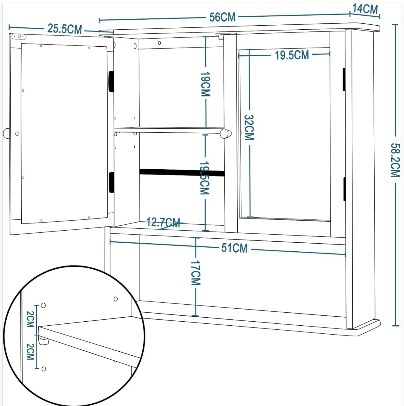
Detailed dimensions diagram of the cabinet, including internal shelf and compartment measurements.
