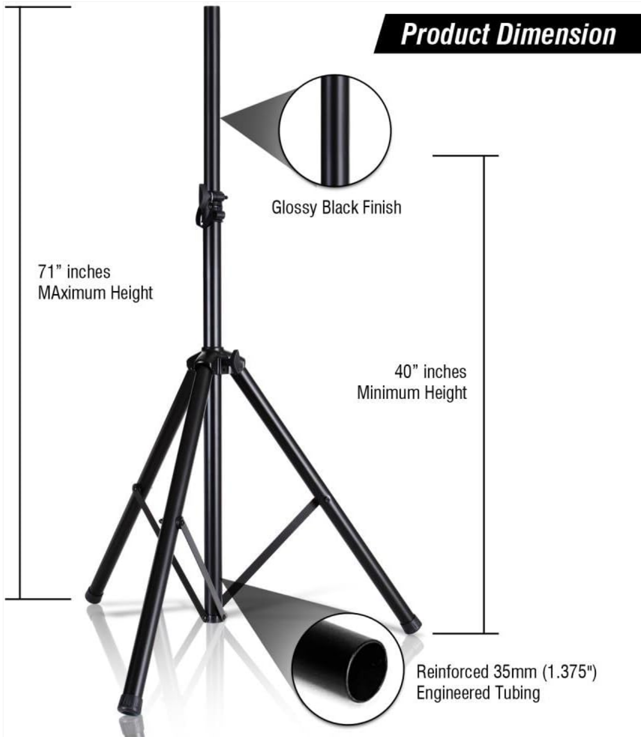
Image: Diagram illustrating the adjustable height range (40" to 71") and reinforced tubing of the Pyle Universal Speaker Stand.
