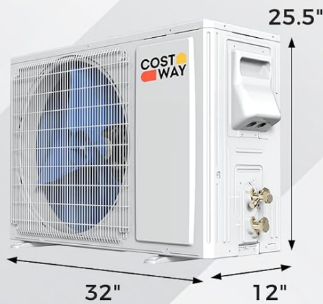
Outdoor Unit
