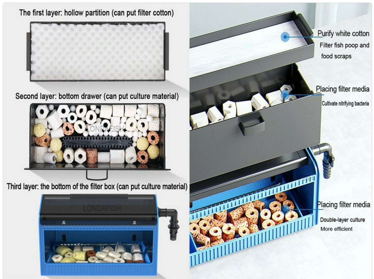
Figure 2: Internal structure of the filter box showing placement of filter cotton and biological media.
