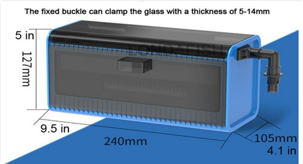
Figure 4: Filter box dimensions.
