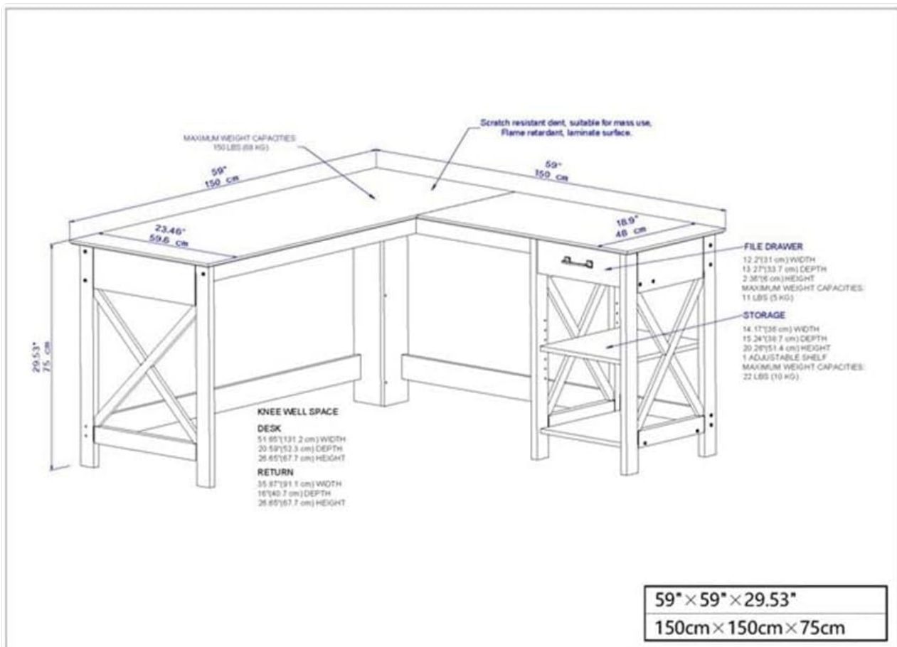
Image 2: Dimensional drawing illustrating the overall dimensions and key sections of the L-shaped desk, including the file drawer, storage, and knee well space.
