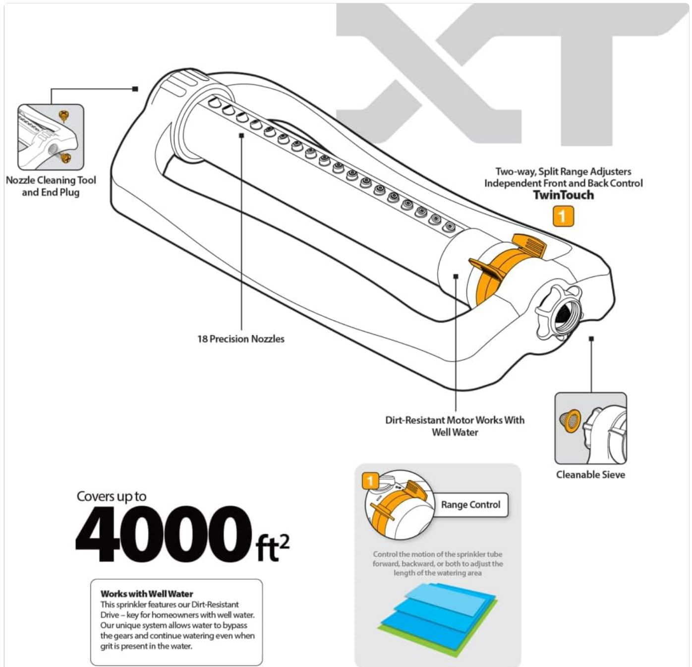
Image: A diagram illustrating the key components of the Melnor sprinkler, including the nozzle cleaning tool, end plug, 18 precision nozzles, dirt-resistant motor, cleanable sieve, and range control with TwinTouch adjusters.
