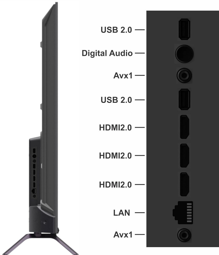
Image: Side view of the Coocaa 55Y72 TV with a detailed diagram of its input and output ports, including USB, Digital Audio, AV, HDMI, and LAN.
