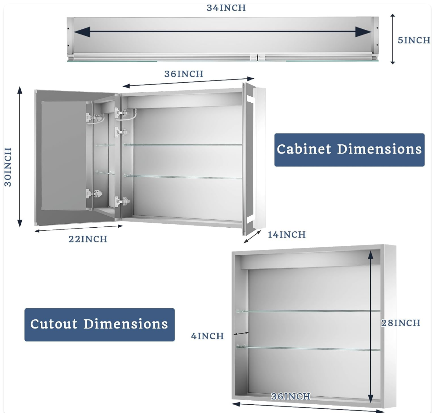
Image: Detailed dimensions for the cabinet and recommended cutout for recessed installation.
