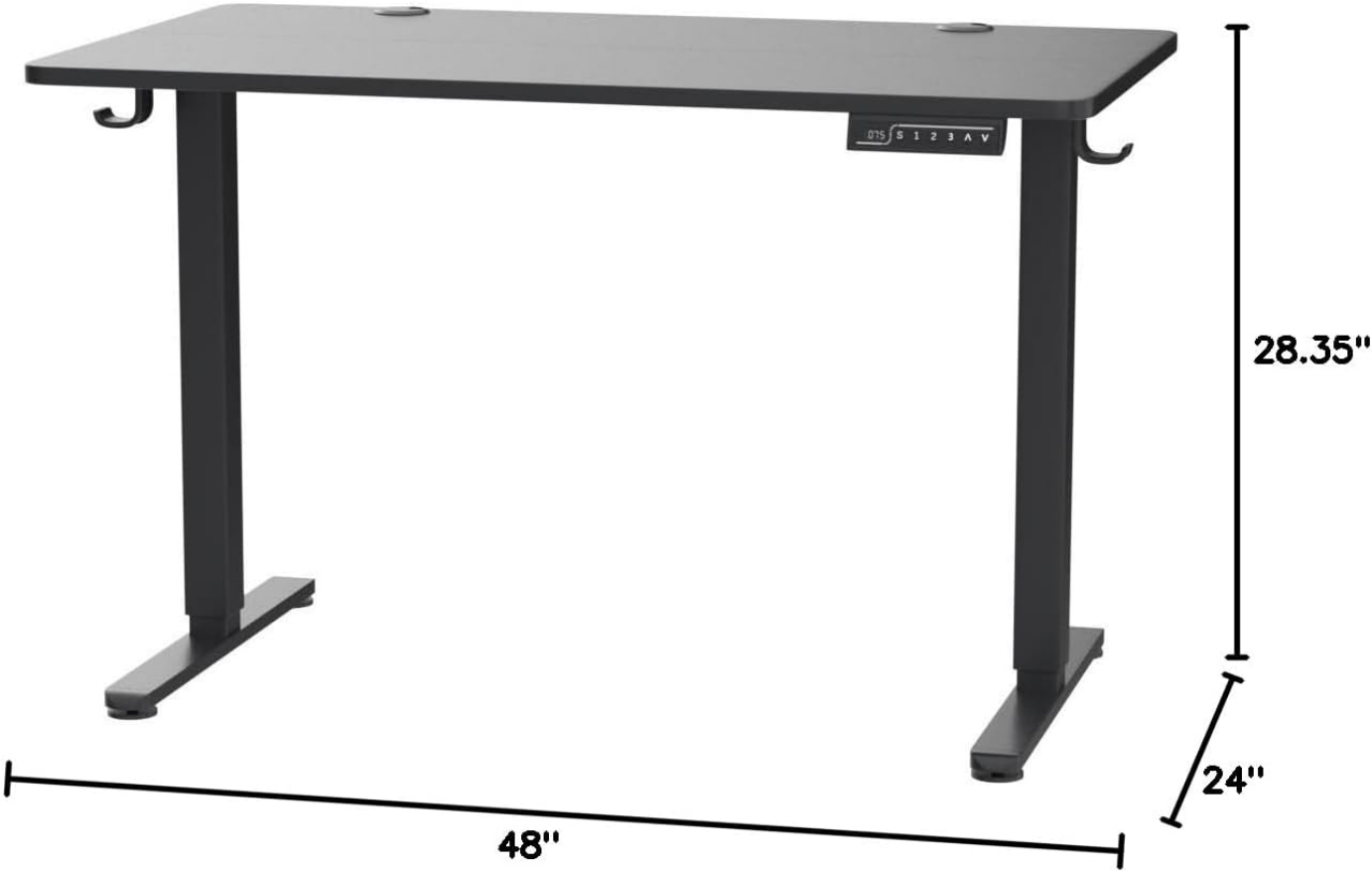
Figure 5: Key dimensions of the ErGear Electric Standing Desk.
