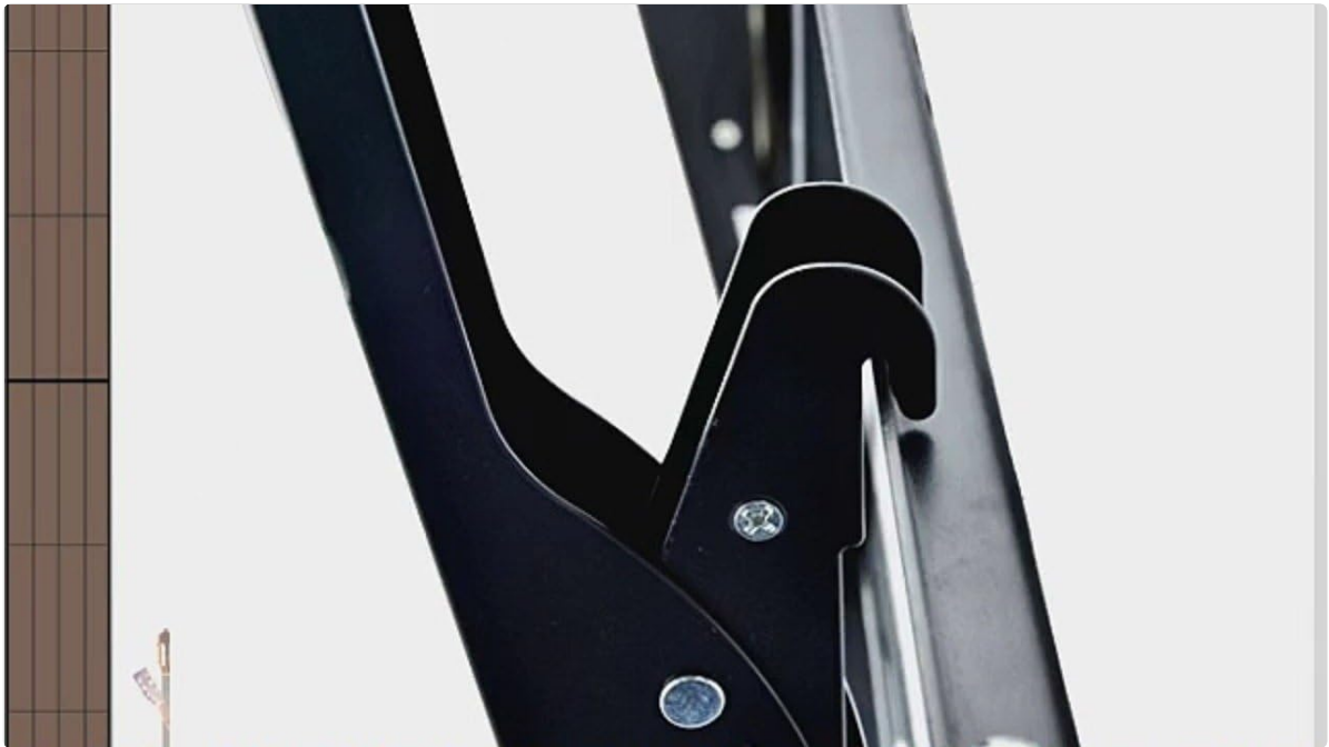
Figure 4: A detailed view of the mount's mechanism, showing how the TV brackets connect to the wall plate and the screw for securing the TV or adjusting the tilt.
