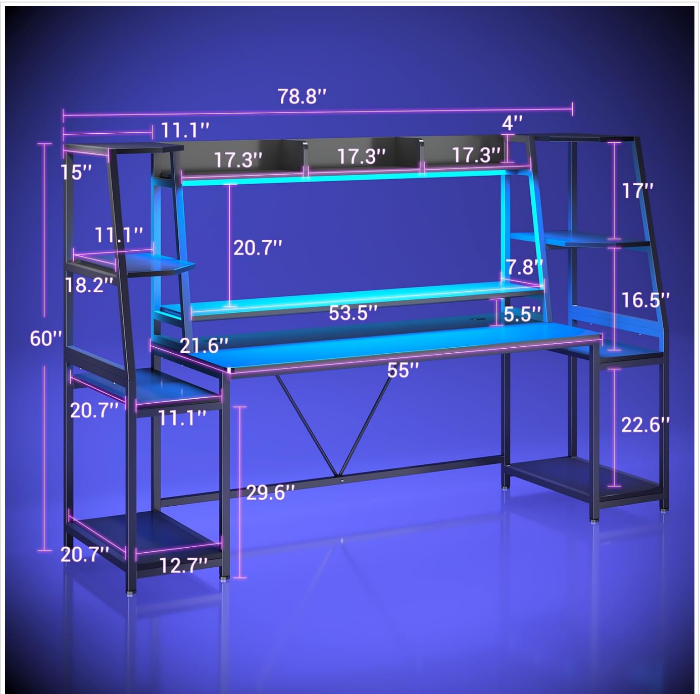
Figure 2: Detailed dimensions of the SEDETA Gaming Desk, including desktop, hutch, and shelf measurements.
