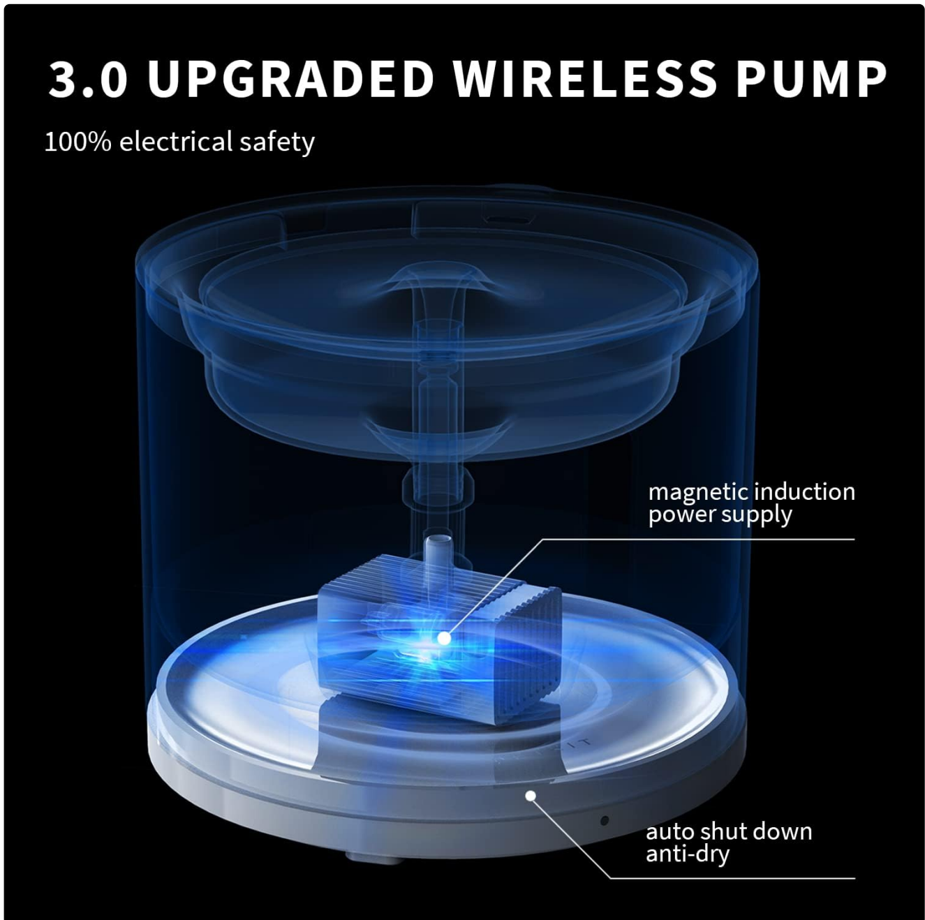
Image: Internal view highlighting the 3.0 upgraded wireless pump with magnetic induction power supply.
