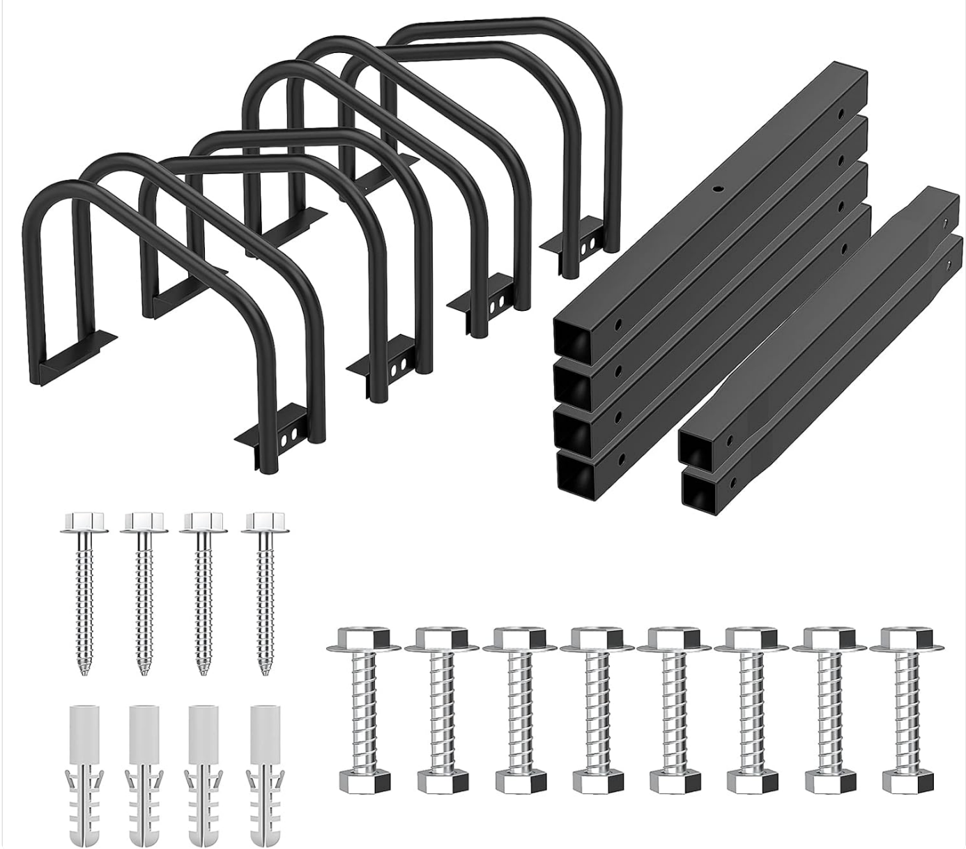
Image: All components included in the WALMANN 4-Bike Floor Bike Stand package: U-shaped bike holders, square base tubes, assembly bolts, and floor mounting anchors.
