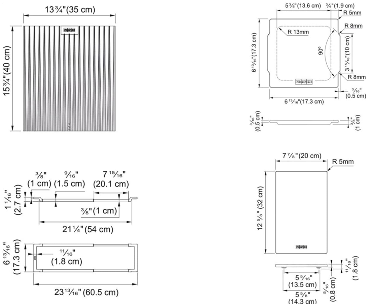
Image: Technical drawing providing detailed dimensions for various components of the Franke All-In Universal Kitchen Sink Accessory System.
