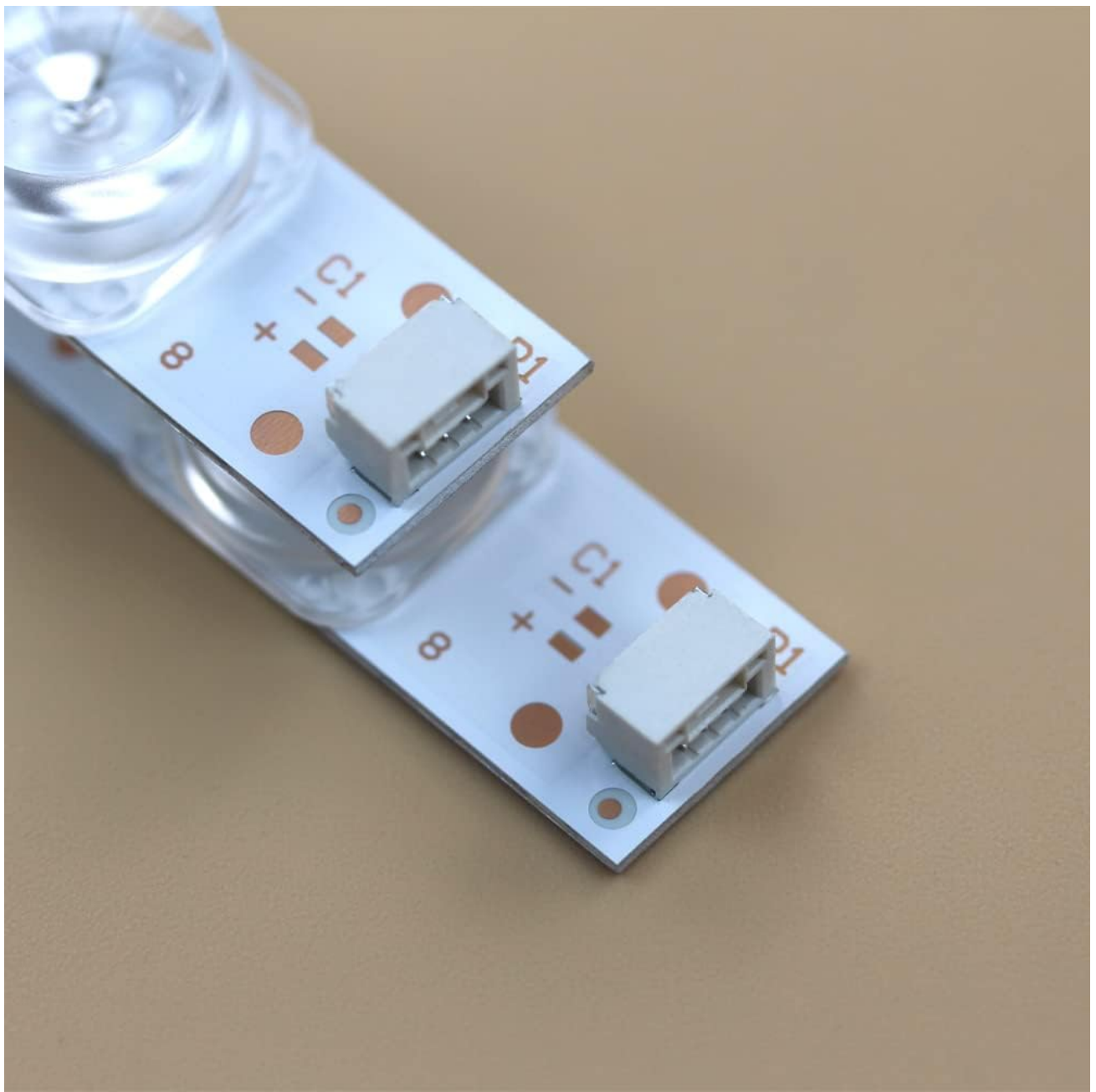
Figure 5.2: Detail of the power connector on the LED backlight strip.
