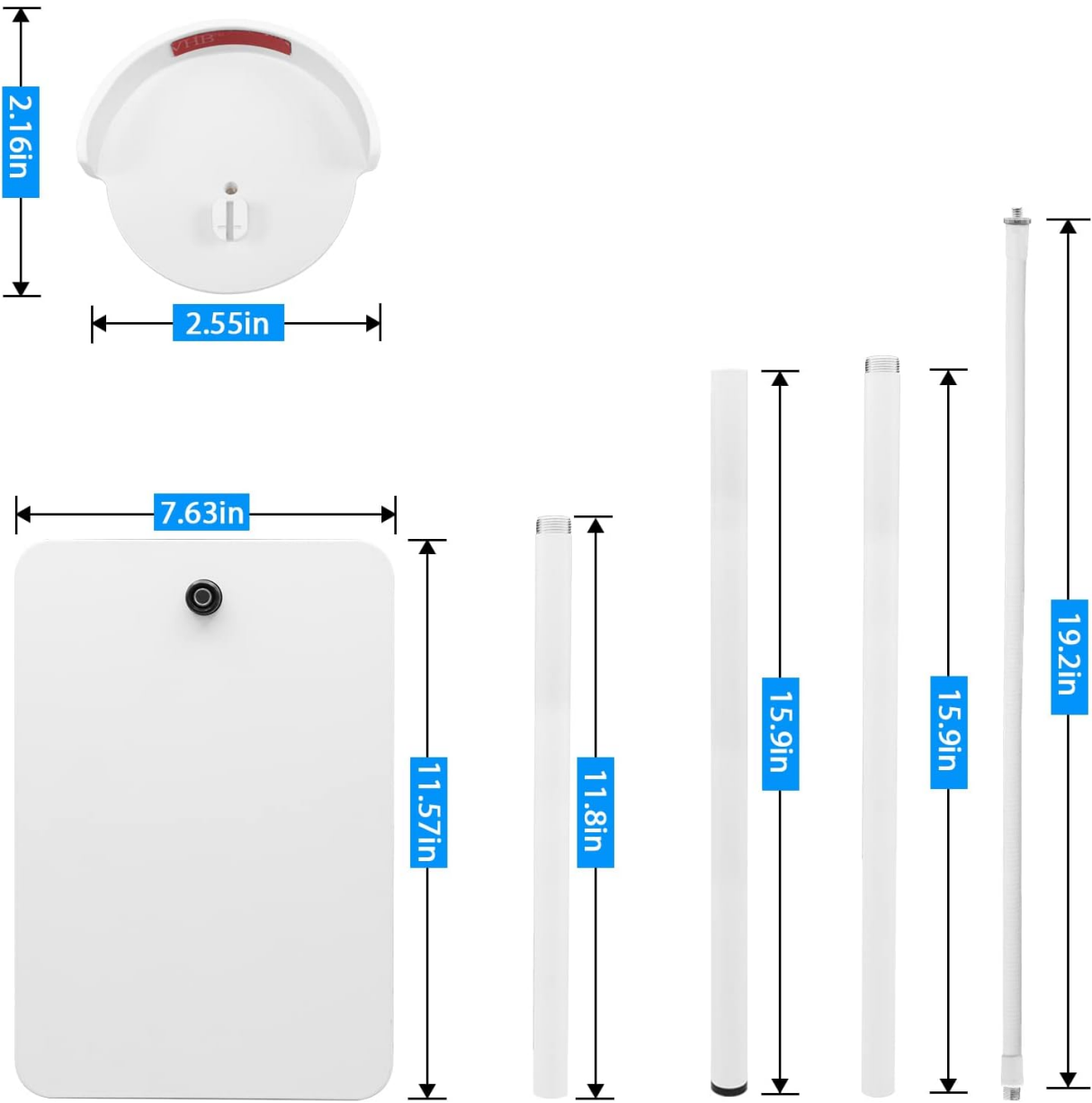
Image: A diagram illustrating the dimensions of the base plate, various rod sections, and the camera mounting bracket.
