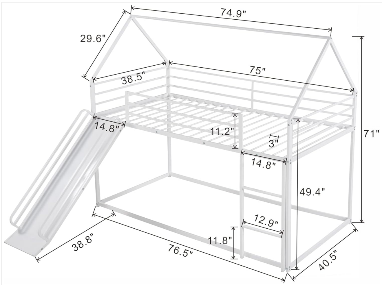
Image: A technical diagram illustrating the precise measurements of the bunk bed, including length, width, height, and distances between components like the slide and ladder.
