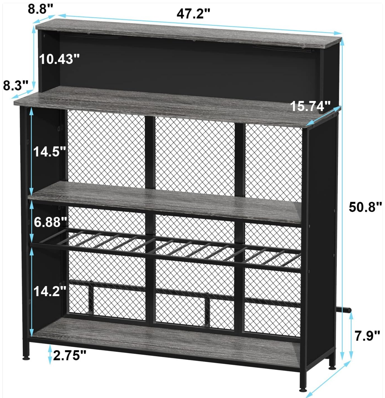
Image: Technical diagram displaying the precise dimensions of the GDLF Home Bar Unit, including height, width, and depth of various sections.
