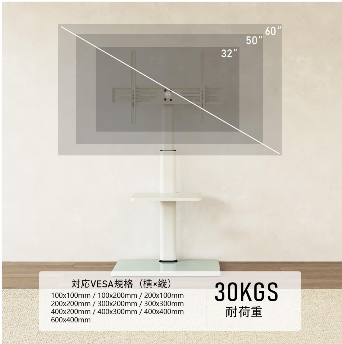
Image: Illustration showing VESA compatibility (100x100mm to 600x400mm) and maximum load capacity of 30kg for the TV.
