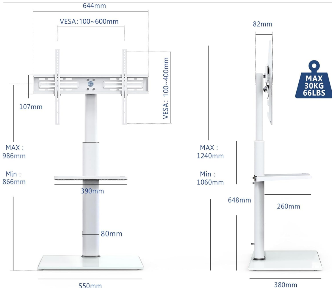
Image: Technical drawing illustrating the detailed dimensions and measurements of the TV stand.
