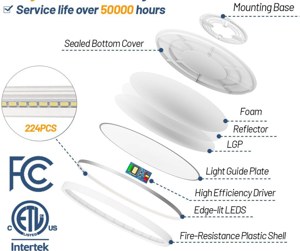
Figure 1: Included components for installation.
