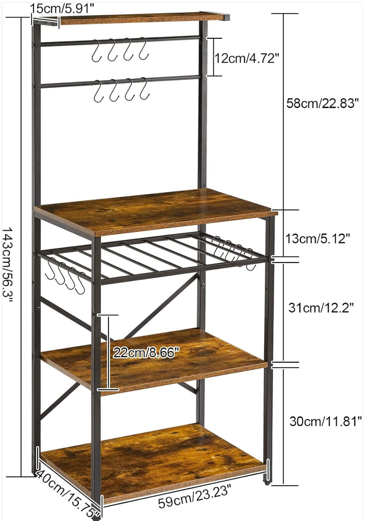
Figure 5: Dimensional diagram of the YMYNY Baker's Rack, illustrating its height, width, and depth, along with shelf spacing.
