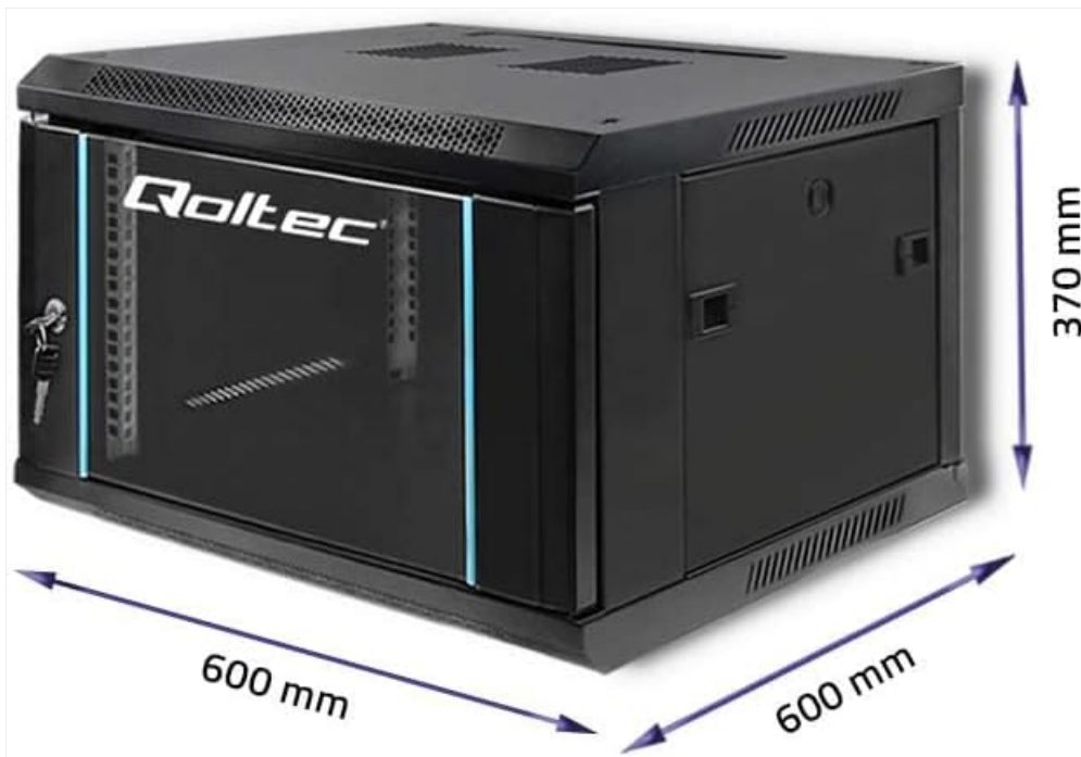
Figure 2: Dimensions of the Qoltec RACK Cabinet. The image illustrates the cabinet's width (600 mm), depth (600 mm), and height (370 mm).
