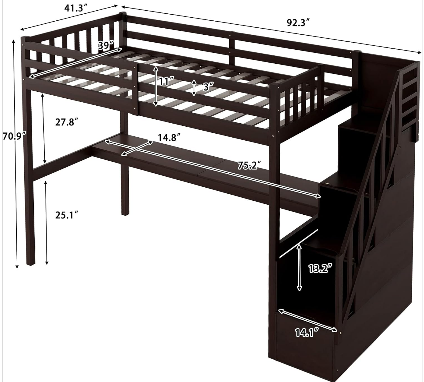
Figure 3.2.2: Dimensional diagram of the SOFTSEA Twin Loft Bed, including bed frame, desk, and staircase measurements.
