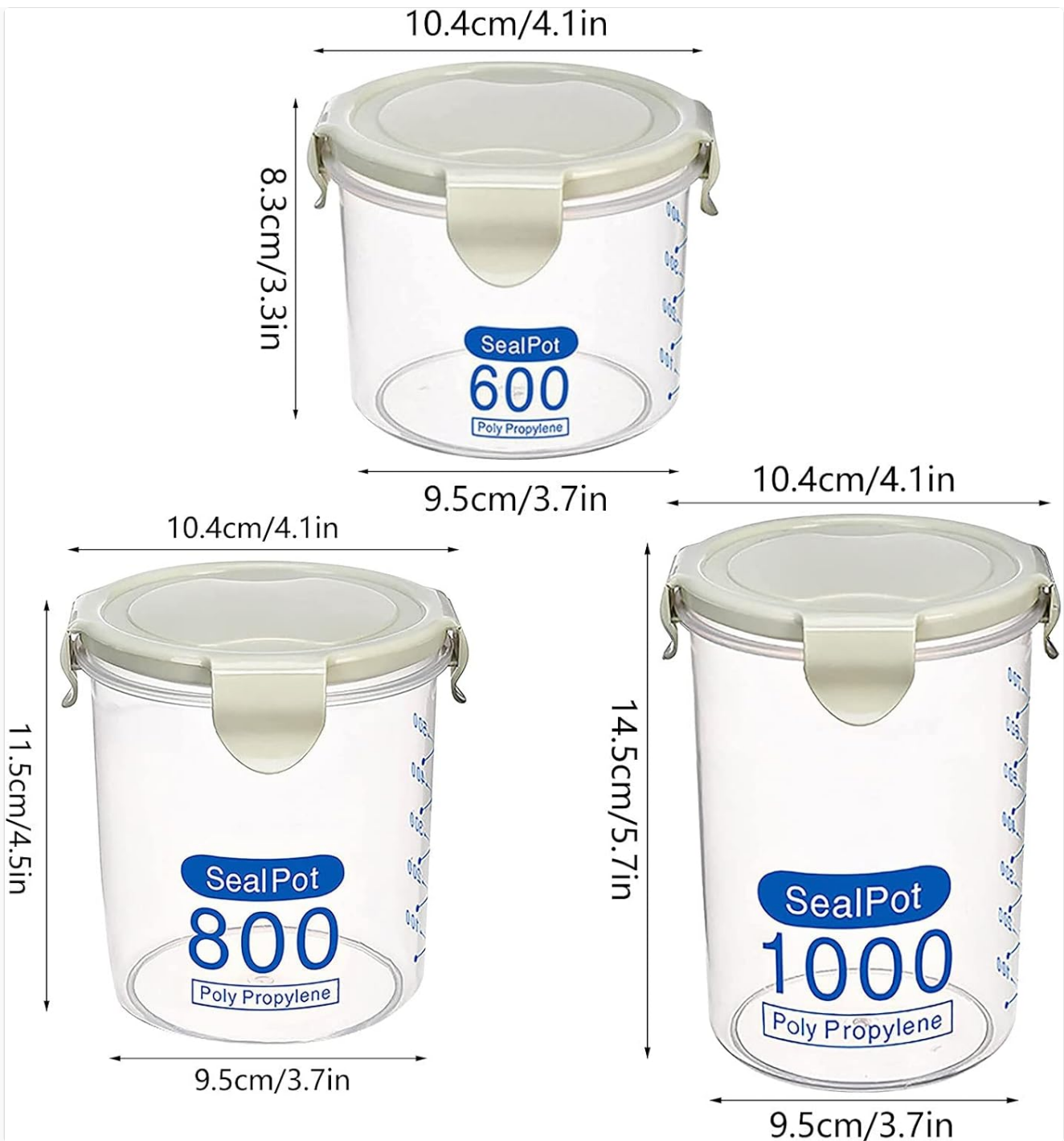
Image: Detailed dimensions for the 600ml, 800ml, and 1000ml containers, including height and diameter.
