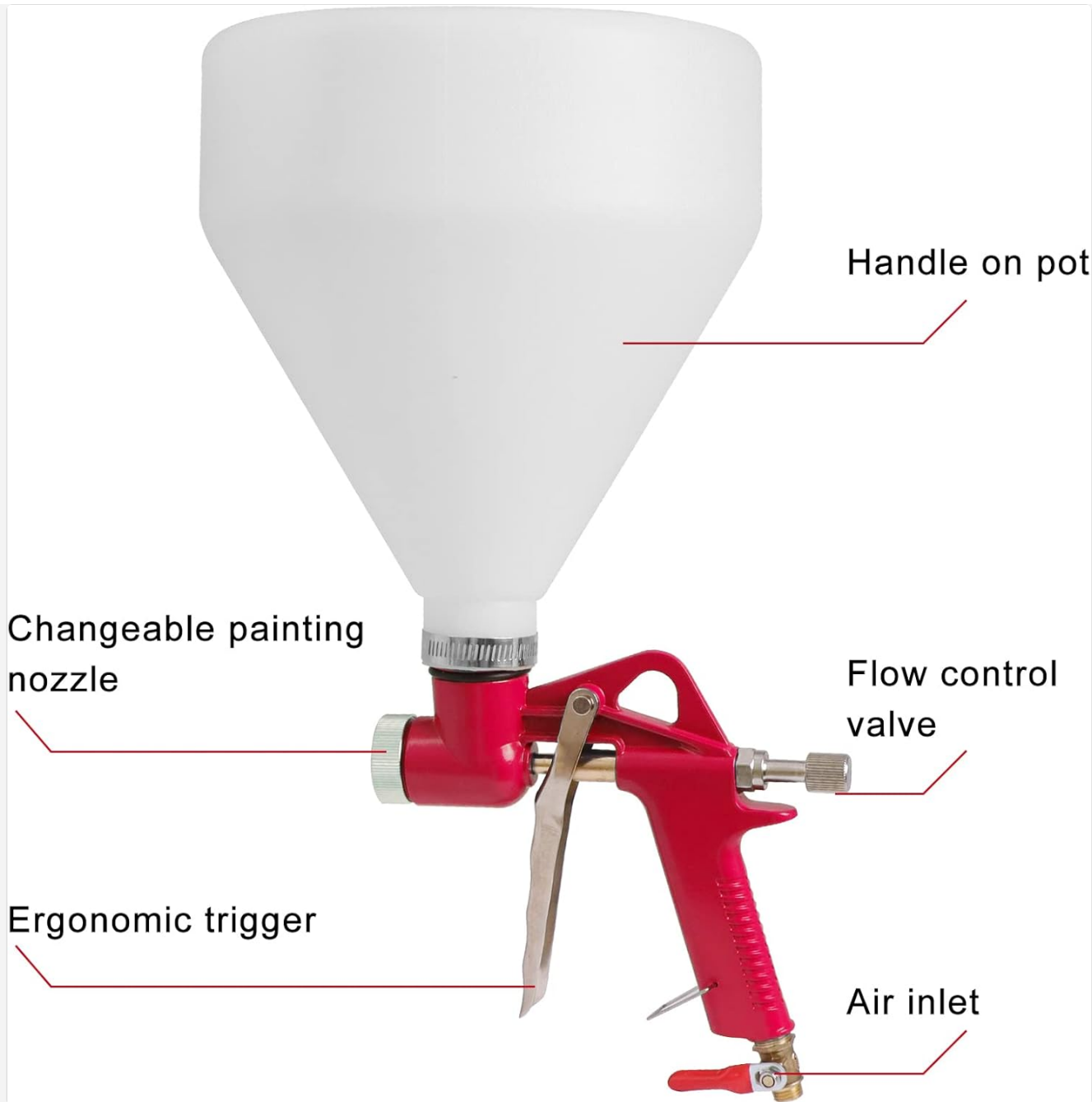
Figure 3.1: Labeled diagram of the texture sprayer, highlighting the handle on the pot, changeable painting nozzle, flow control valve, ergonomic trigger, and air inlet.
