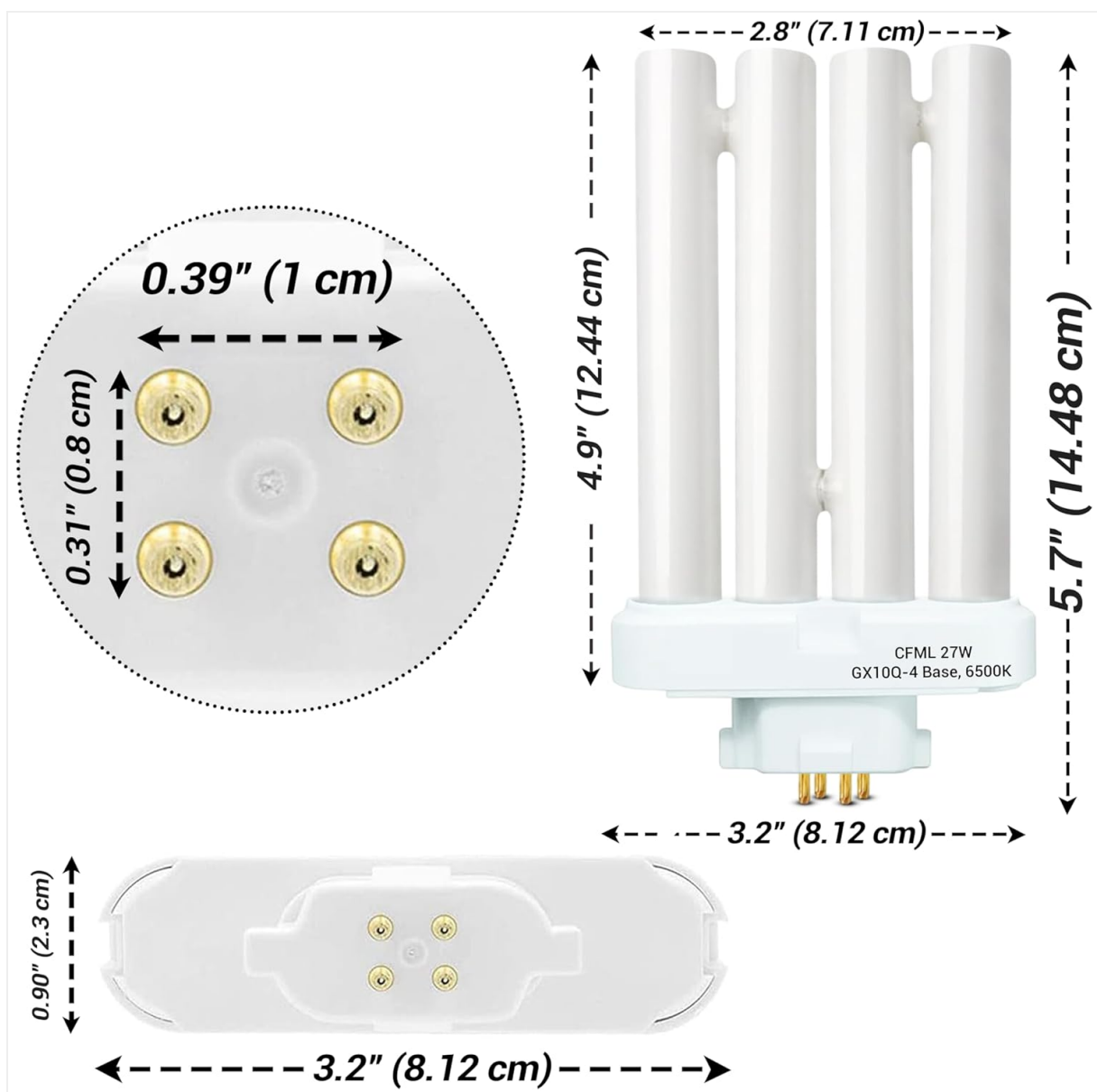
Image: Detailed diagram illustrating the dimensions of the ARSUK 27W CFL bulb, including its length, width, and the specific measurements of the GX10Q-4 base pins.
