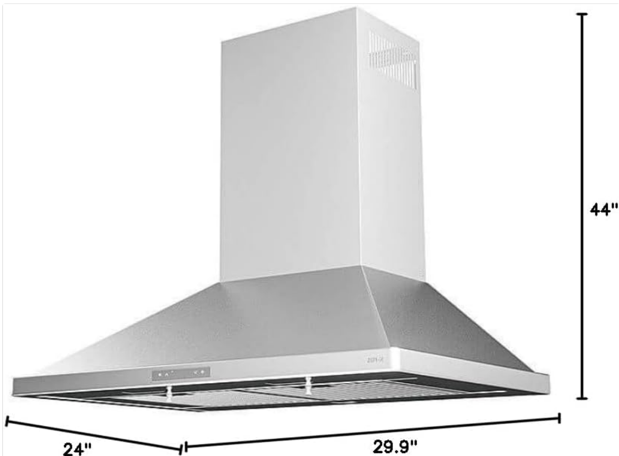
Figure 5: Product dimensions.
