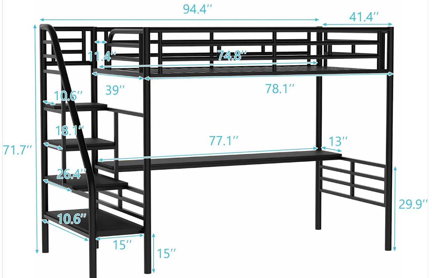
Figure 2.1: This diagram illustrates the precise measurements of the loft bed, including length, width, height, and dimensions of the desk and stairs.
