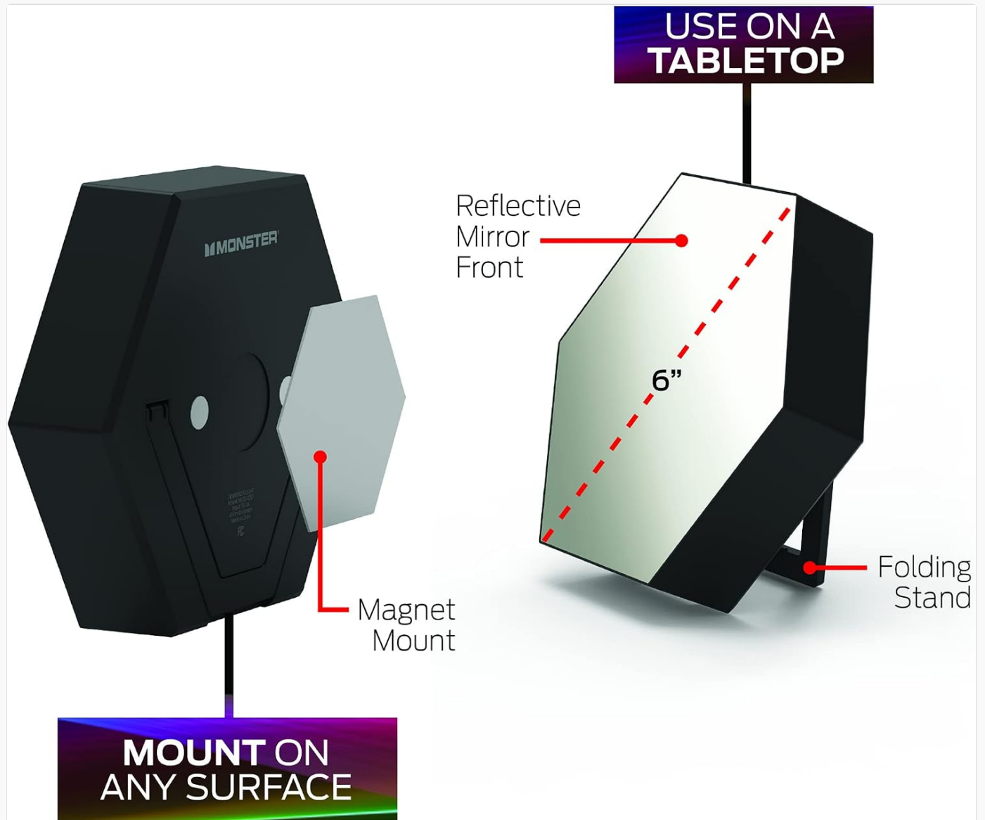
Image: Illustration detailing the magnetic mount for wall installation and the folding stand for tabletop placement of the light.
