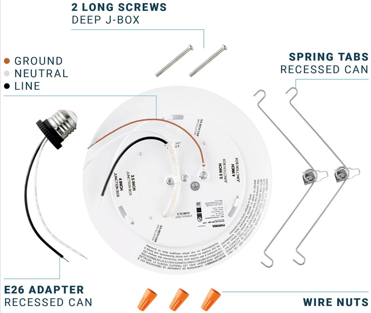
Image 3.1: All accessories included for installation, such as the E26 adapter, wire nuts, screws, and spring tabs.
