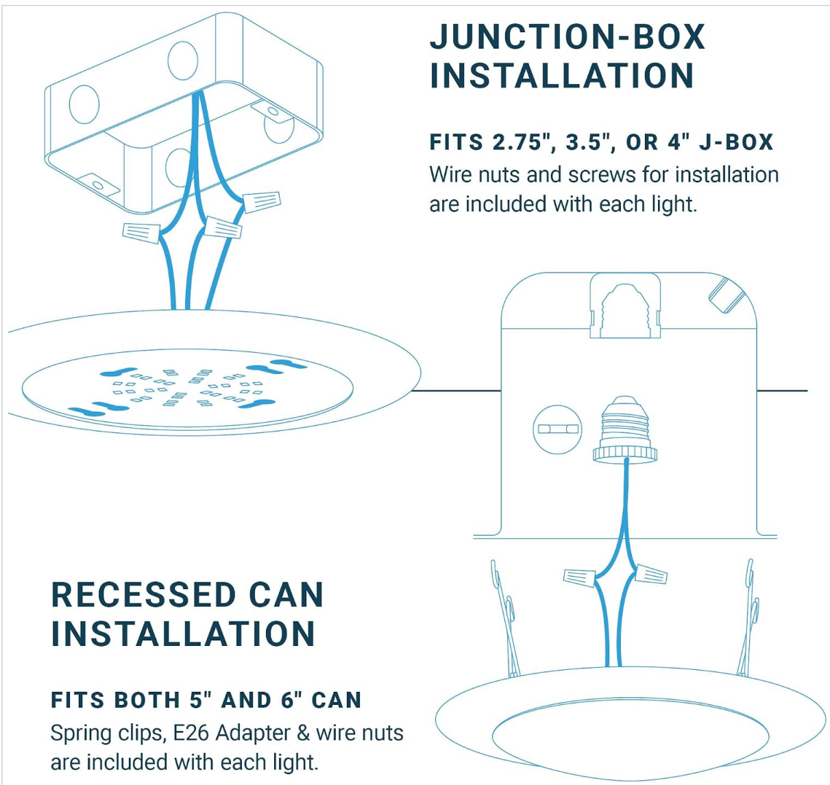
Image 5.2: Illustration of wiring for junction box installation (top) and recessed can installation (bottom).
