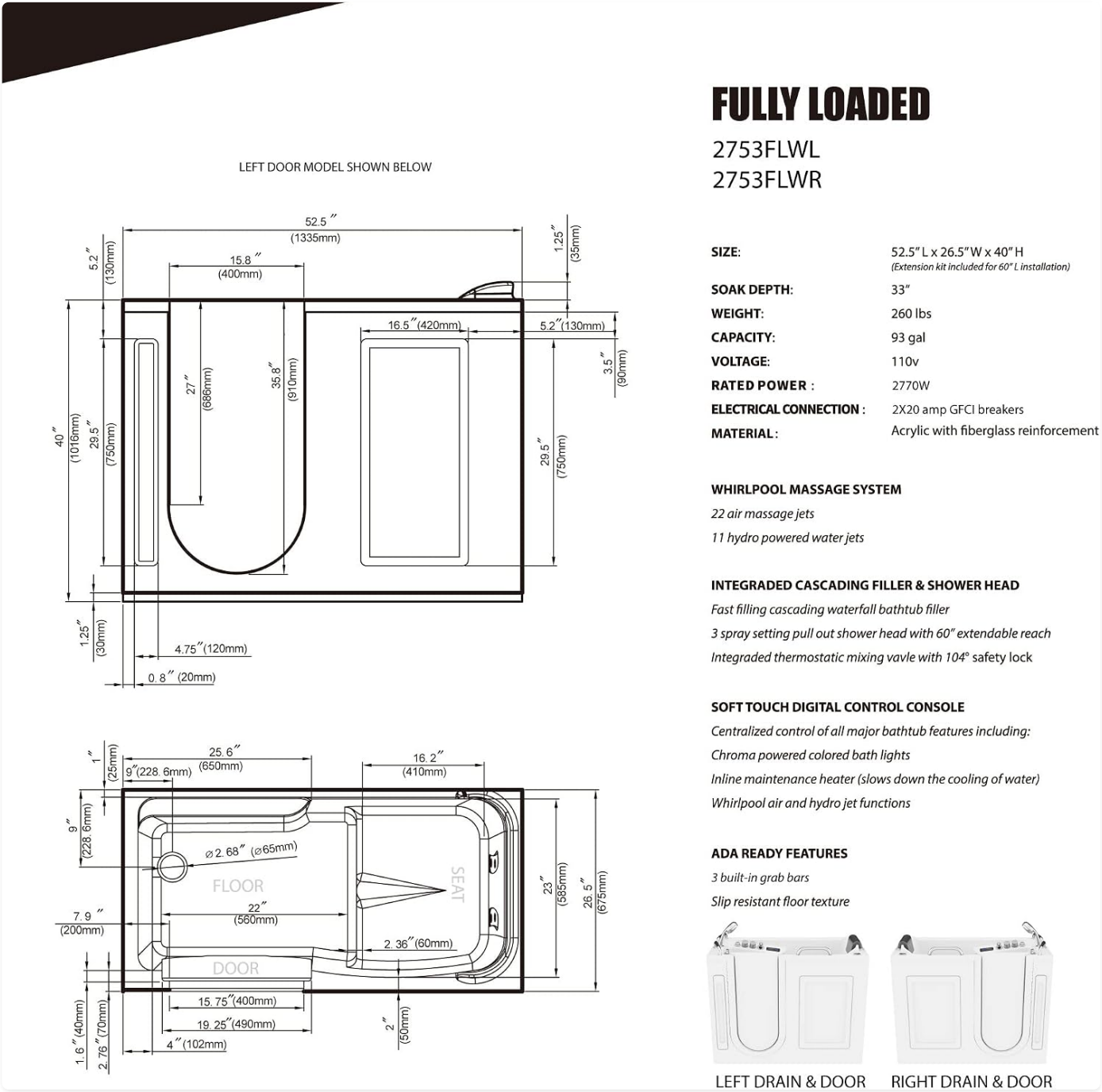
Figure 3.1: Detailed technical drawing with dimensions and specifications crucial for proper installation planning.
