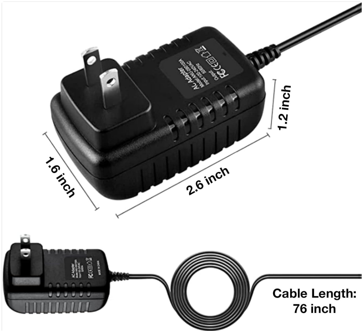
Figure 3.2: The AC adapter with indicated dimensions (2.6 inches length, 1.6 inches width, 1.2 inches height) and a cable length of 76 inches.
