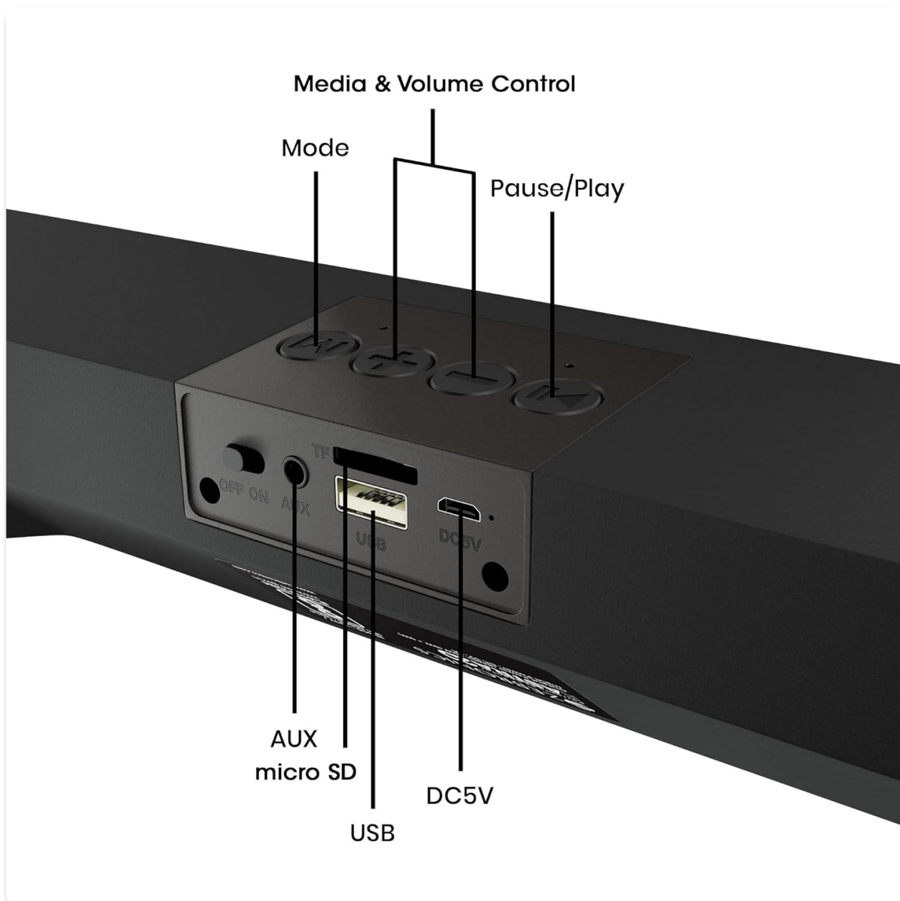
Figure 5: Control panel and connectivity ports.
