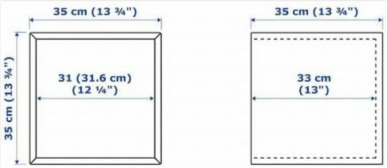
Figure 5: Detailed dimensions of the EKET cabinet.
