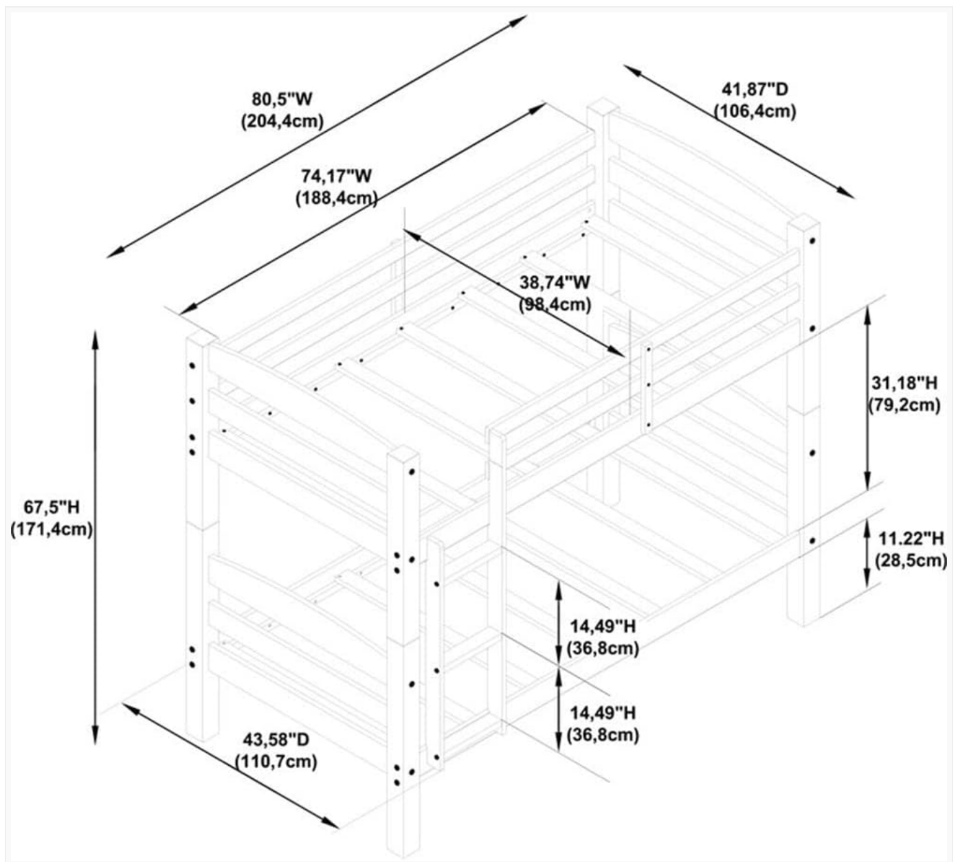
Figure 2: Dimensional diagram of the bunk bed, illustrating overall size and component measurements.
