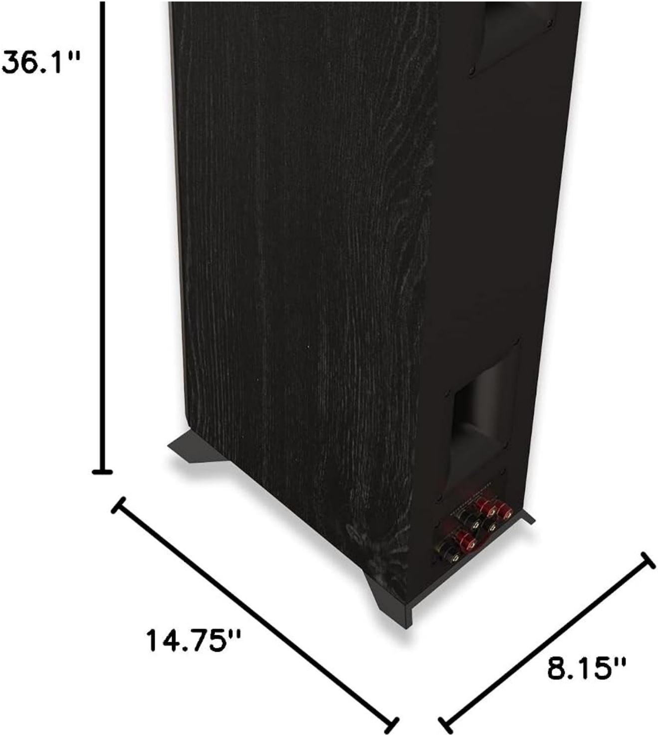
Image: Diagram illustrating the dimensions of the Klipsch RP-5000F II speaker.
