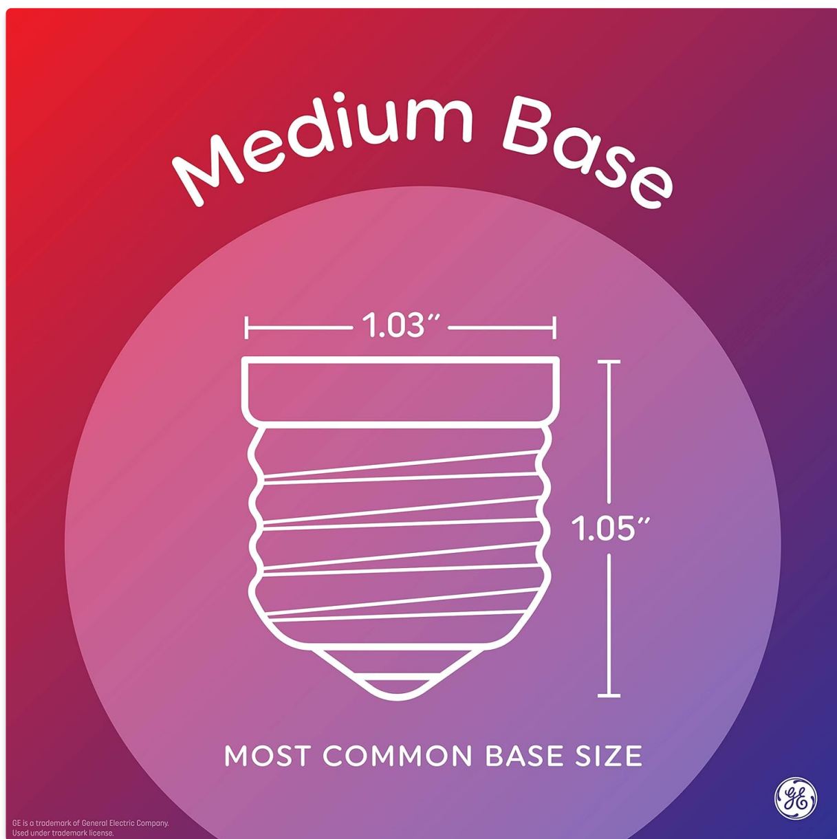
Figure 7: Dimensions of the E26 Medium Base, the most common base size for light bulbs.
