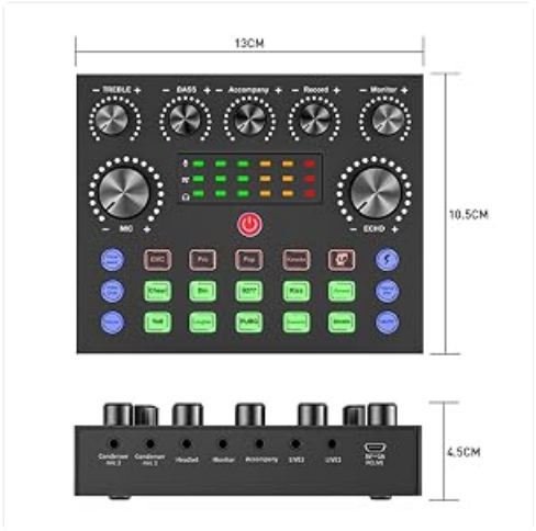
Image: A technical diagram illustrating the precise dimensions of the V8S Audio Mixer, including its length, width, and height, for accurate spatial planning.
