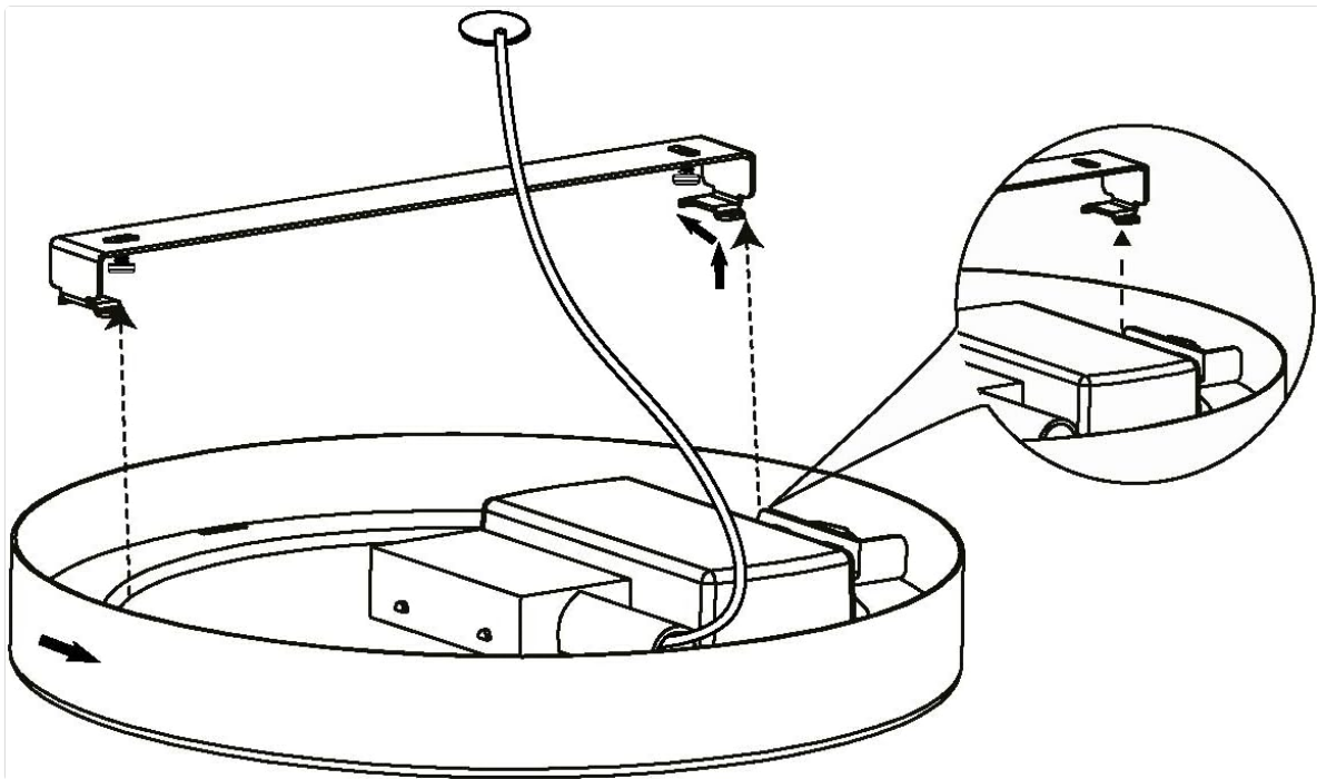
Image 4.1: Installation diagram showing how the light fixture attaches to the mounting bracket.
