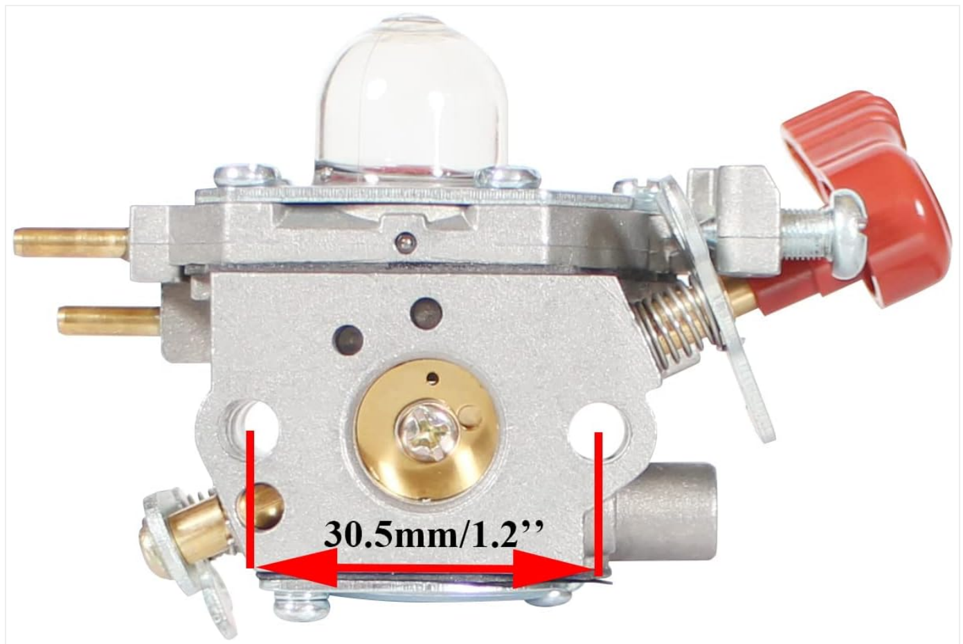
Image 4.1: View of the carburetor showing the mounting hole distance of 30.5mm (1.2 inches), important for proper fitment.
