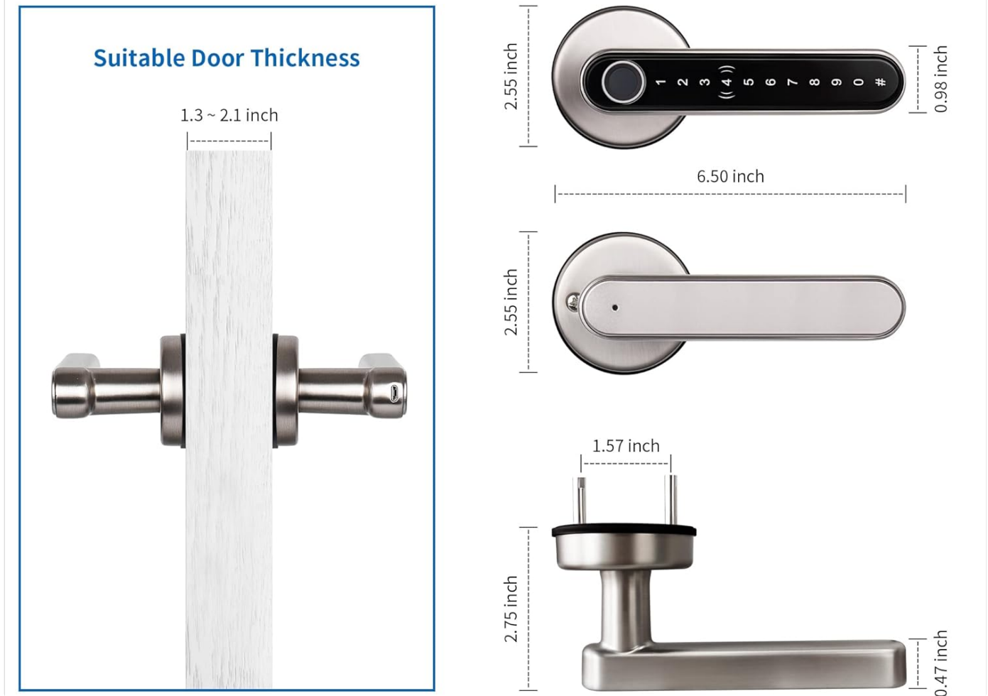
Figure 4: Door thickness compatibility and lock dimensions.
