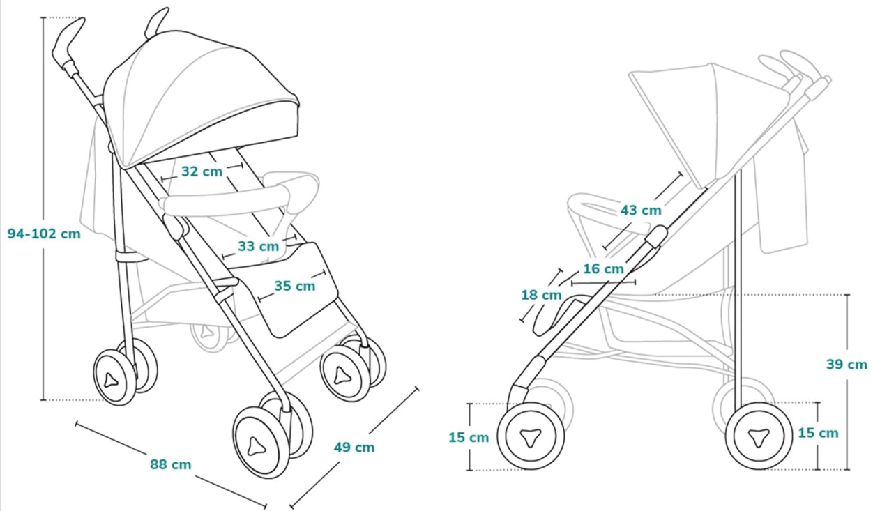
Image 8.1: Technical diagram illustrating the various dimensions of the Irma Stroller when unfolded and folded.
