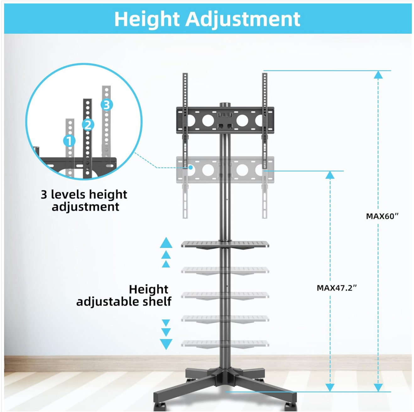
Figure 5: Illustration of TV and shelf height adjustment capabilities.
