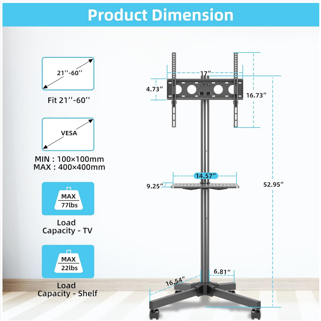
Figure 3: Detailed product dimensions and load capacities.
