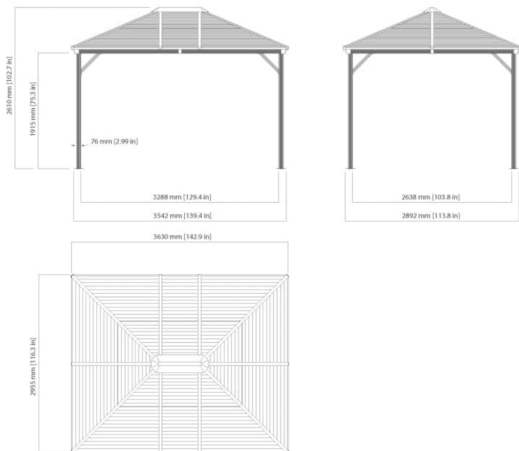
Image 3.1: Technical drawing illustrating the dimensions of the Sojag Ventura Gazebo, useful for site planning.
