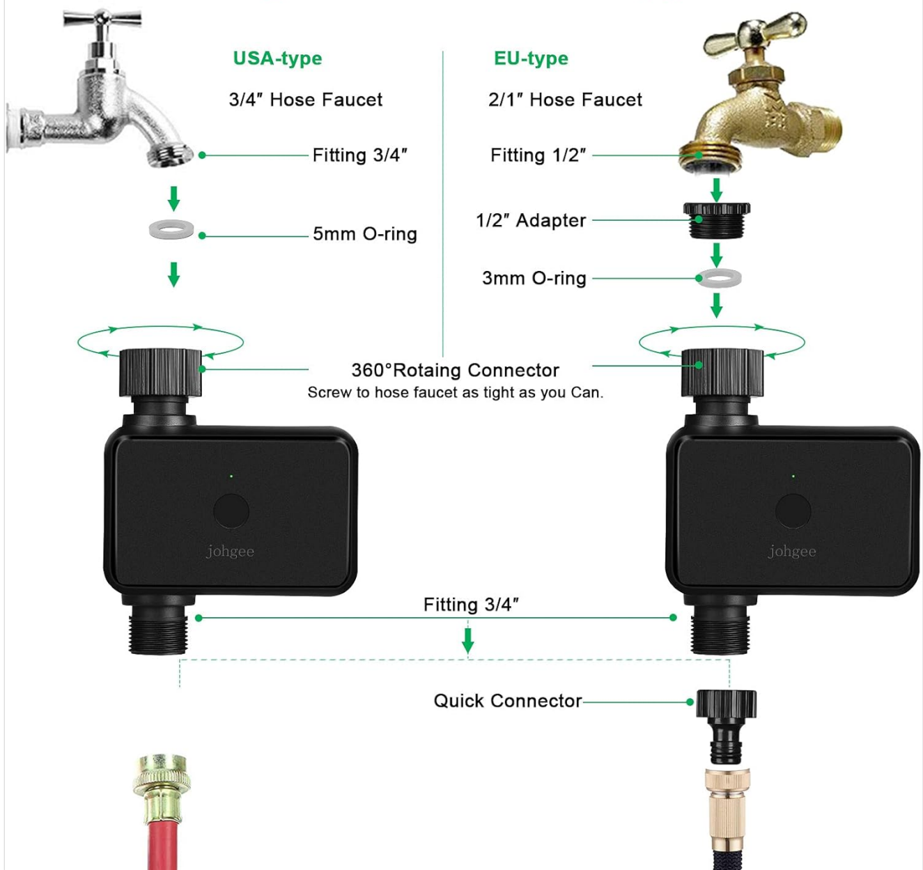
Image: Detailed diagram illustrating the connection of the water timer to both USA-type (3/4" hose faucet) and EU-type (2/1" hose faucet) standards, including the use of O-rings and adapters.
