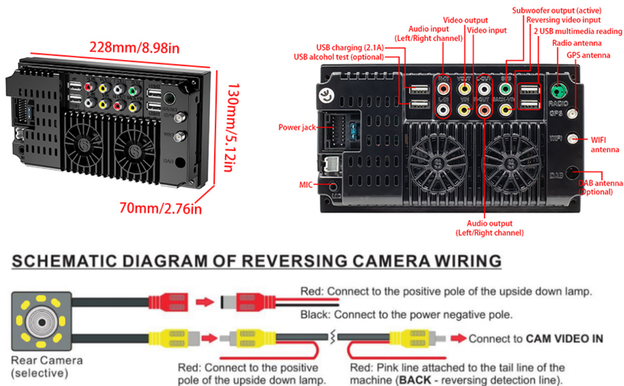
Image: Schematic diagram illustrating the various input and output ports on the rear of the car stereo, including power, audio, video, USB, GPS, WiFi, and the specific wiring for the reversing camera.
