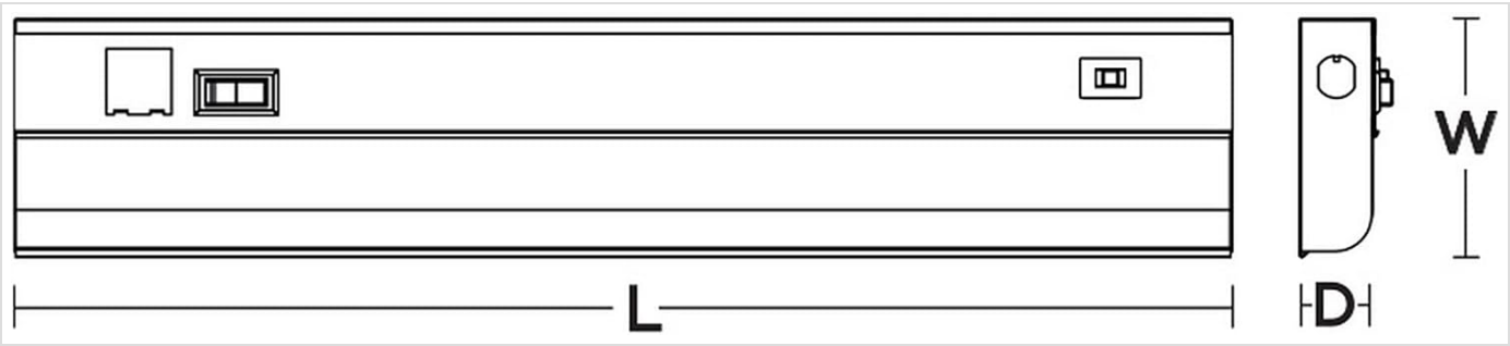
Figure 3: Dimensional diagram of the AFX T5L 2 fixture, illustrating its length (L), width (W), and depth (D) for installation planning.
